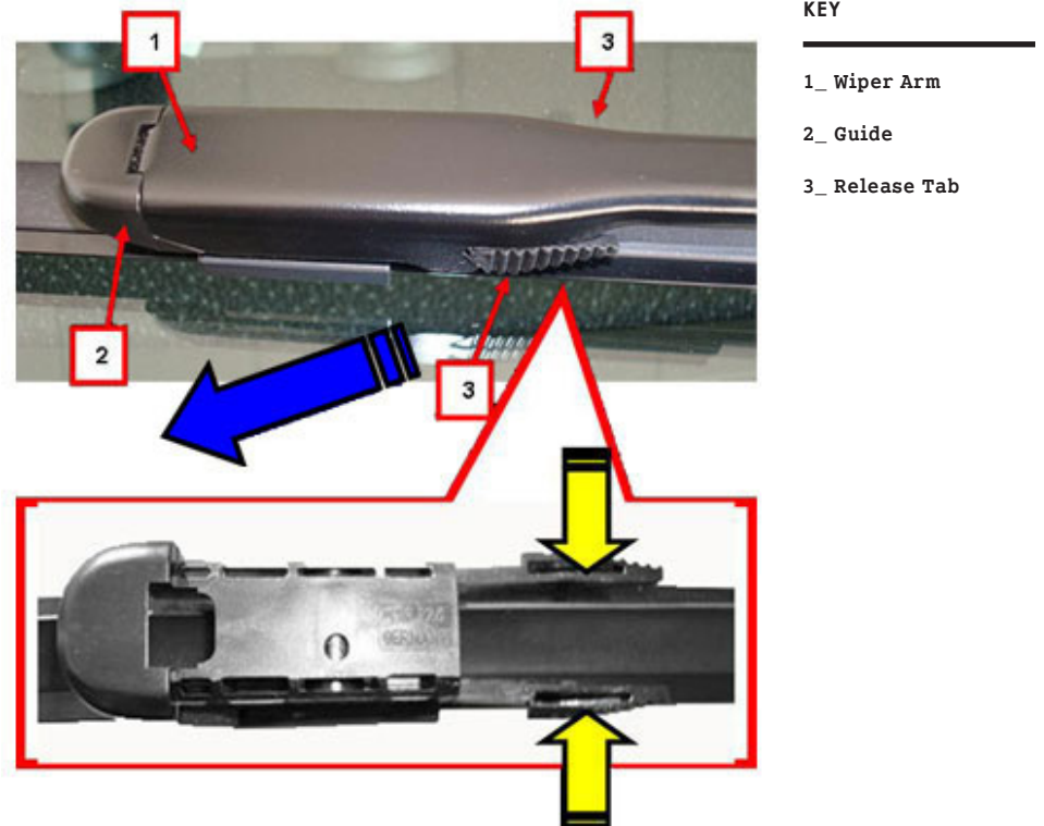
FIGURE A - FRONT WINDSHIELD WIPER
